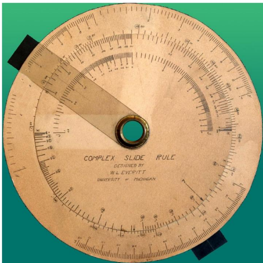
THE EVERITT COMPLEX HYPERBOLIC SLIDE RULE OF 1924
