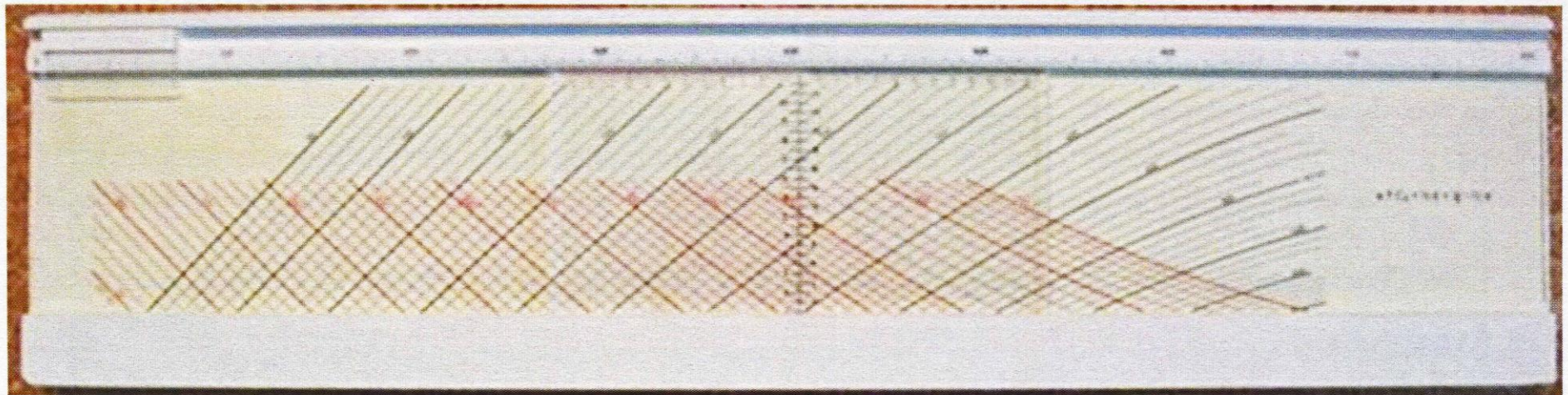
FIGURE 5. Aristo 90120 "Rivera Patent"
